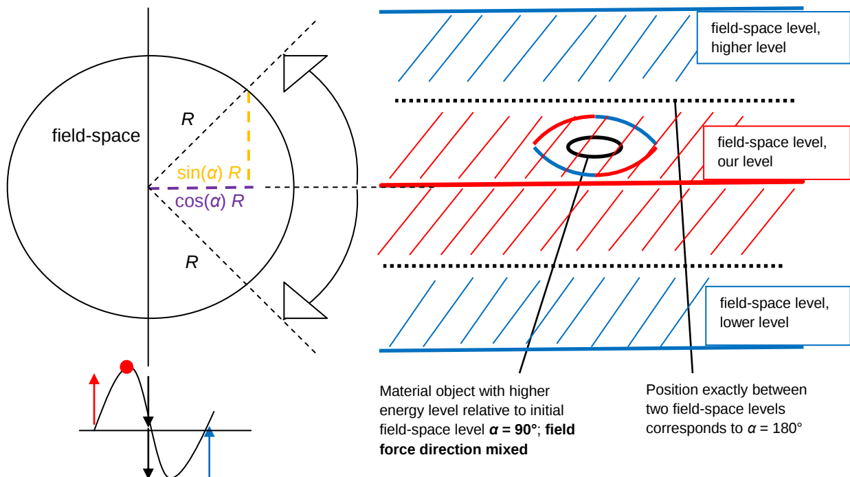
Figure 4.3B: The displacement of an object between the initial and higher field-space levels; field forces reflected between them for m_{obj} \cos(\alpha = 90^\circ)
