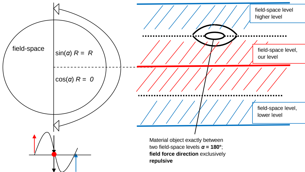
Figure 4.3C: The displacement of an object exactly between the initial and higher field-space levels; field forces act repulsively for m_{obj} \cos(\alpha = 180^\circ)
